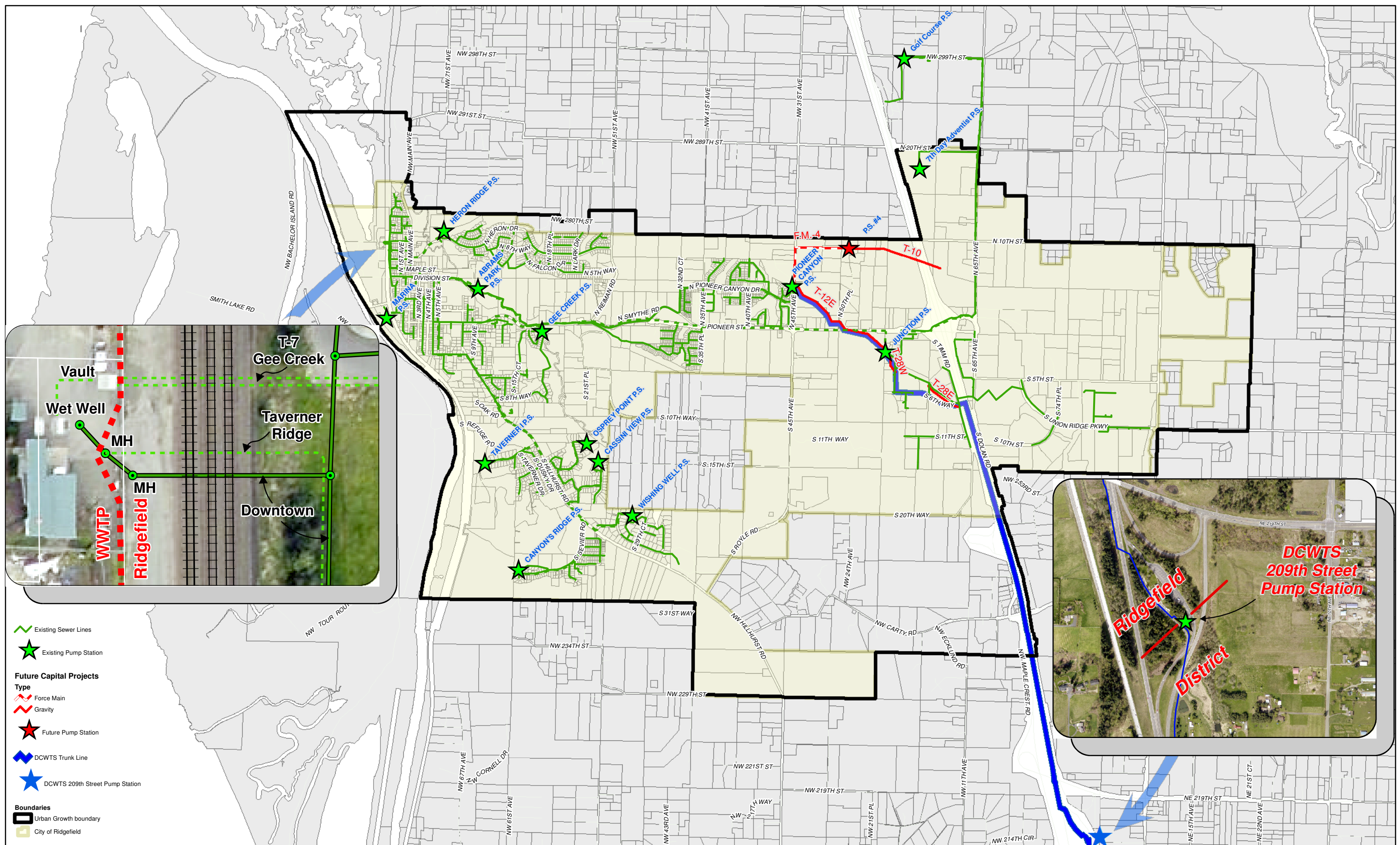
Exhibit B Map 1 - Ridgefield Sewer Collection System Infrastructure
